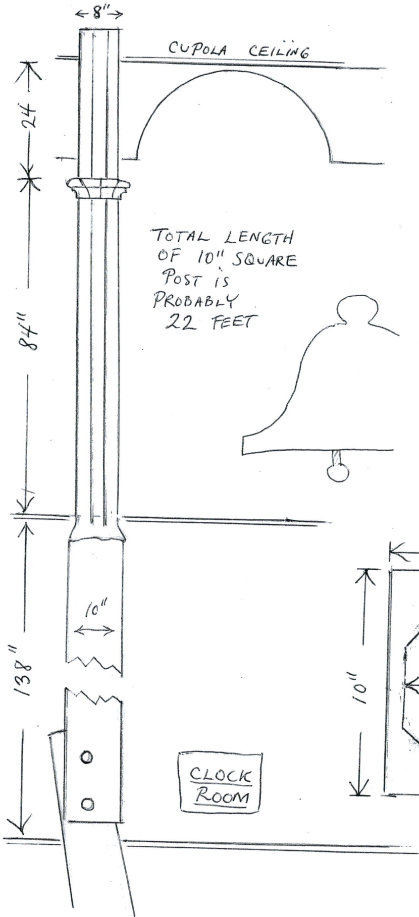
OCTAGONAL POST CUT FROM 10" SQUARE POST.
