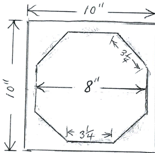
OCTAGONAL POST CUT FROM 10" SQUARE POST.
